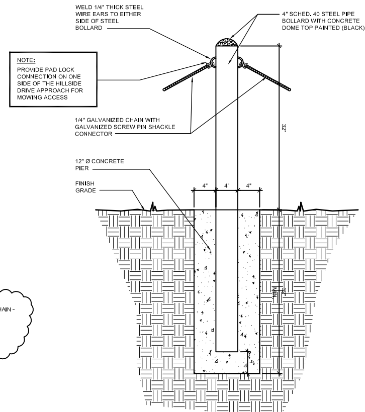
1 BOLLARD DETAIL 1 1/2" = 1'-0"
